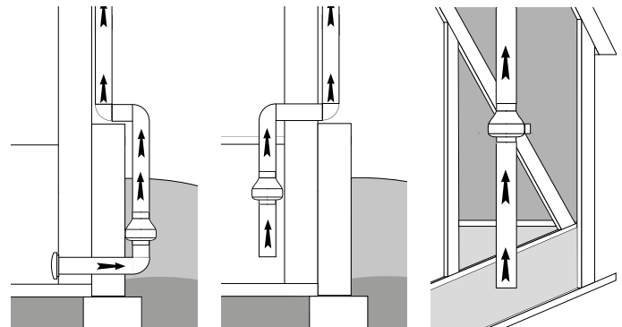
Outside installation
