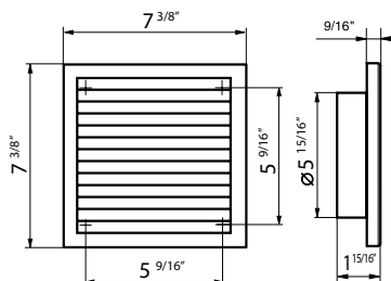
MV 150 Vs
